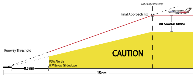
Figure 10-22 ILS Approach PDA Alert Threshold
