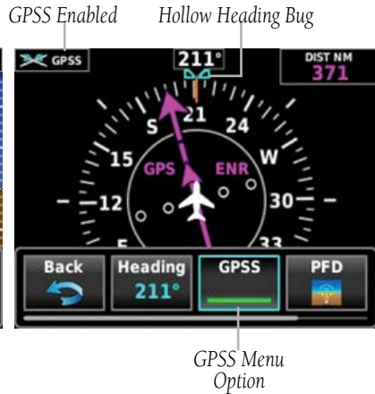
Figure 4-4 GPSS Enabled (HSI Page)
